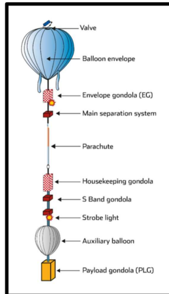
Fig. 4. Scheme of a Zero Pressure Balloon used within the HEMERA programme.
