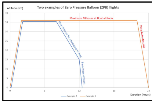
Fig. 5. The plot shows the altitude in km of the Zero Pressure Balloon used within the HEMERA programme as a function of the flight time in hours.
